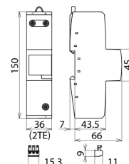
Dimension drawing DGPM 1 255 FM
