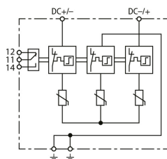
Basic circuit diagram DCB YPV 1200 FM
