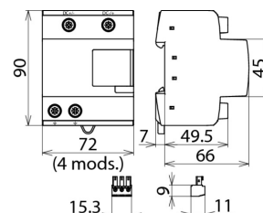
Dimension drawing DCB YPV 1200 FM
