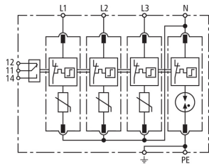
Basic circuit diagram DG M TT 275 CN FM
