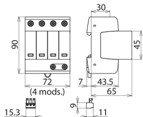
Dimension drawing DG M TT 275 CN FM
