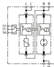
Basic circuit diagram DG MP TT 2P 385 FM
