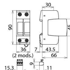
Dimension drawing DG MP TT 2P 385 FM
