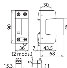
Dimension drawing VT1 M 12.5 TT 2P 385 FM
