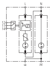
Basic circuit diagram VT1 M 12.5 TT 2P 385 FM
