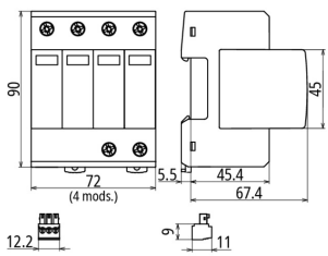
Dimension drawing VT2 M TT 320 CN FM
